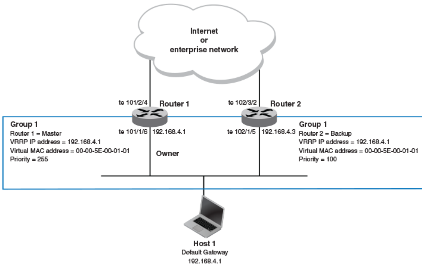
FIGURE 33 Devices configured as VRRP virtual routers for redundant network access for Host 1
